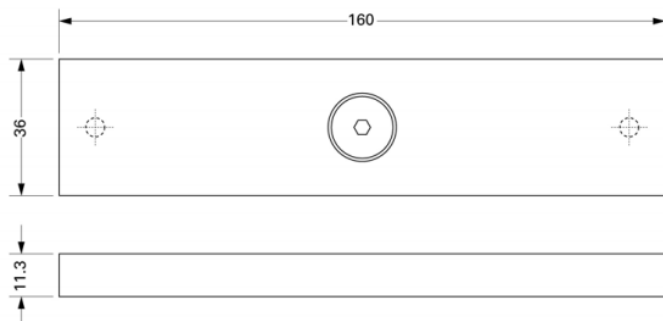
Armature Unit
